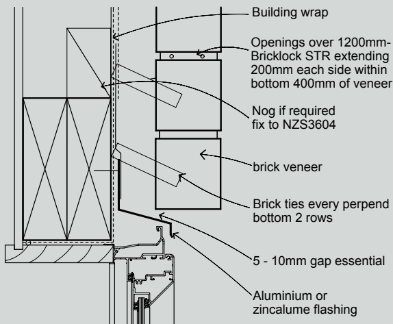
Fig C. Steel-less Lintel- Standard Stretcher
