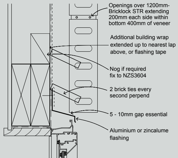
Fig D. Steel-less Lintel- Soldier Course
