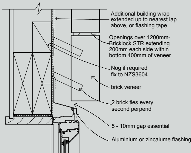
Fig E. Double Height Brick
