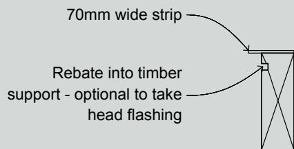
Section Through Temporary Lintel Support
