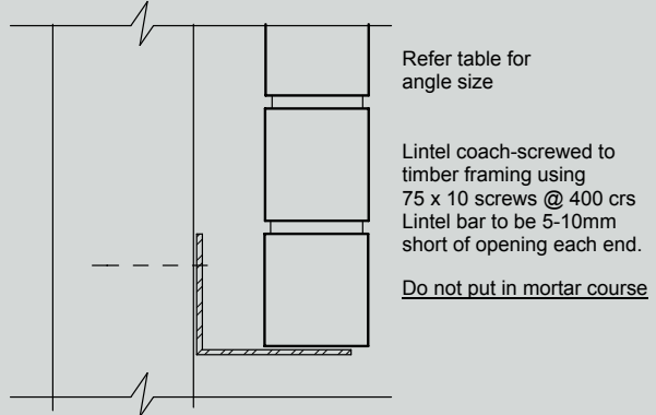
Fig B. Lintel- Fixed to framing
