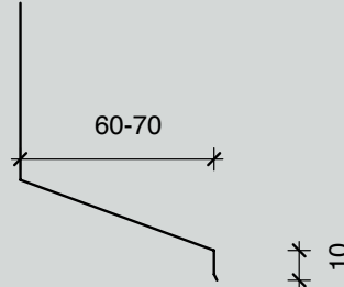
Fig F. Head Flashing
