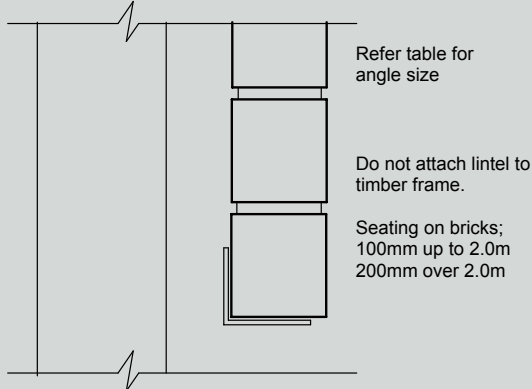
Fig A. Lintel- Traditional
